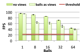
(a) Frames/second comparison
