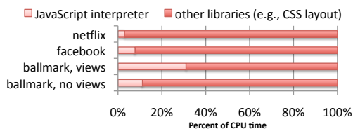
(b) Relative JavaScript execution time
