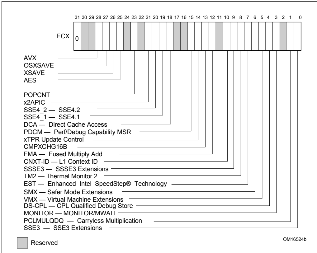
Figure 3-7. Feature Information Returned in the ECX Register
