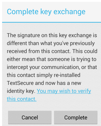
Fig. 2. TextSecure warning for key changes: the user must either accept the new key by selecting “complete”, or perform manual verification [31].
